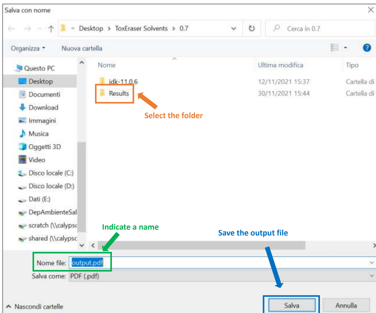
Figure 6: The figure shows how to select the output directory
